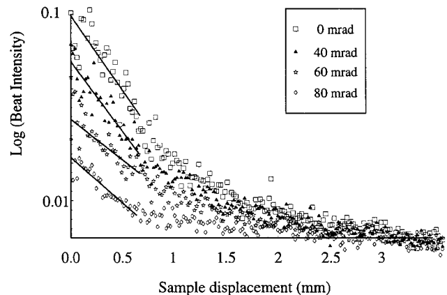
Fig. 2. Heterodyne beat intensity as a function of sample displacement for selected scattering angles (points, data; lines, exponential fits). The sample used to obtain these data was 6.1- \mu\text{m} polystyrene microspheres suspended in water.
