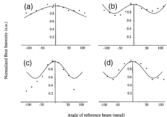
Fig. 3. Angular distributions for the fitted A parameter for media consisting of (a) 1.9-, (b) 4.6-, and (c) 6.1- \mu\text{m} -diameter microspheres. Increasing the coherence length of the source alters the angular scattering distribution (d) of the 6.1- \mu\text{m} microspheres.
