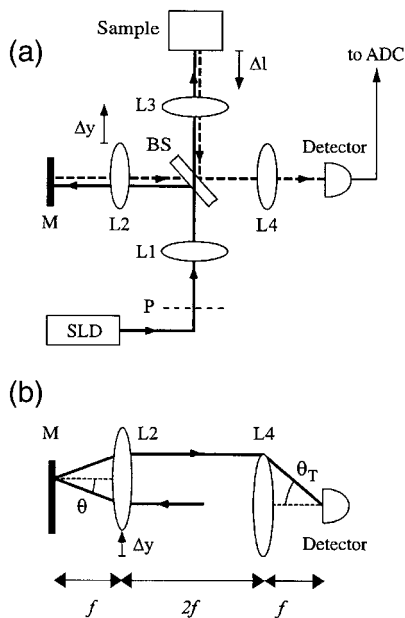
Fig. 1. (a) Schematic of the interferometer system. The photocurrent is digitized by an analog-to-digital converter (ADC) and recorded with a PC. See text for other definitions. (b) Ray-trace diagram showing the effect of translating lens L2 by a distance \Delta y , resulting in the reference field's crossing the detector at an angle \theta_T .
