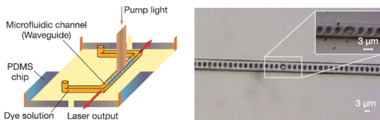
FIGURE 2. An optofluidic distributed-feedback (DFB) dye laser consists of a microfluidic channel with a distributed-feedback Bragg grating structure (left). A dye solution, which acts as both the core of the optical waveguide and the gain medium, can be introduced into the structure via the channel. An excitation pump light field is incident on the laser structure. The laser wavelength can be tuned by changing the dye choice or by stretching/compressing the flexible PDMS to change the periodicity of the DFB structure (right). 2
