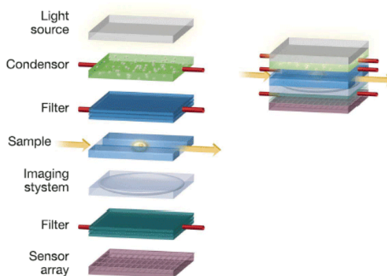
FIGURE 1. In an adjustable-focal-depth optofluidic transmission microscope, the light source, the condenser, the spectral filters, and the imaging system are replaced with optofluidic components, which can enable the creation of cheap, easily configurable, and compact microscope systems.
