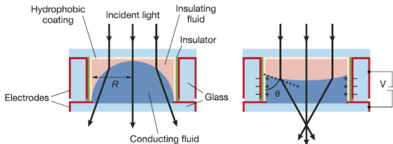
FIGURE 3. In an electrowetting-based optofluidic lens (left), the application of a voltage alters the solid-liquid interfacial tension, and with that the contact angle (right). 6
